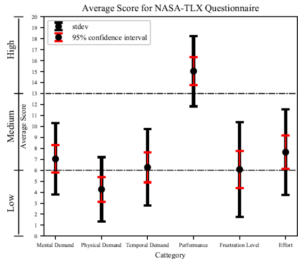
Figure 7: NASA-TLX questions.
