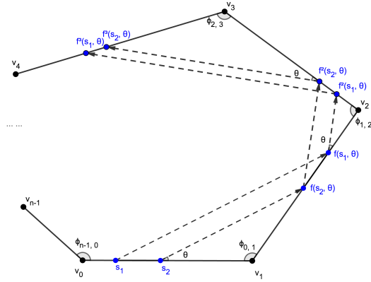
Fig. 10: The notation setup for the proof of contracting cycle in a convex polygon.
