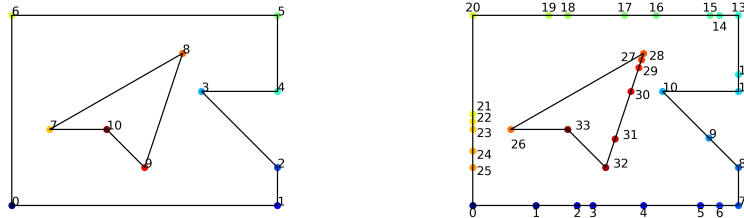
Fig. 5: An example partition for a polygon with holes; our discretization scheme extends naturally to handle static obstacles.
